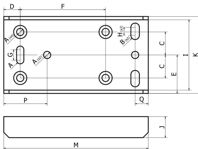
PF56413 - Adapting plate for tube mounting
